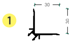
LDD CLAD CORNER MALE
